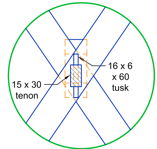
Detail 2 Scale 1:3
