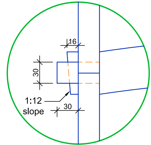
Detail 1 Scale 1:3
