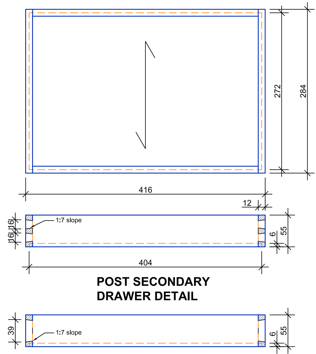
SECONDARY DRAWER DETAIL
