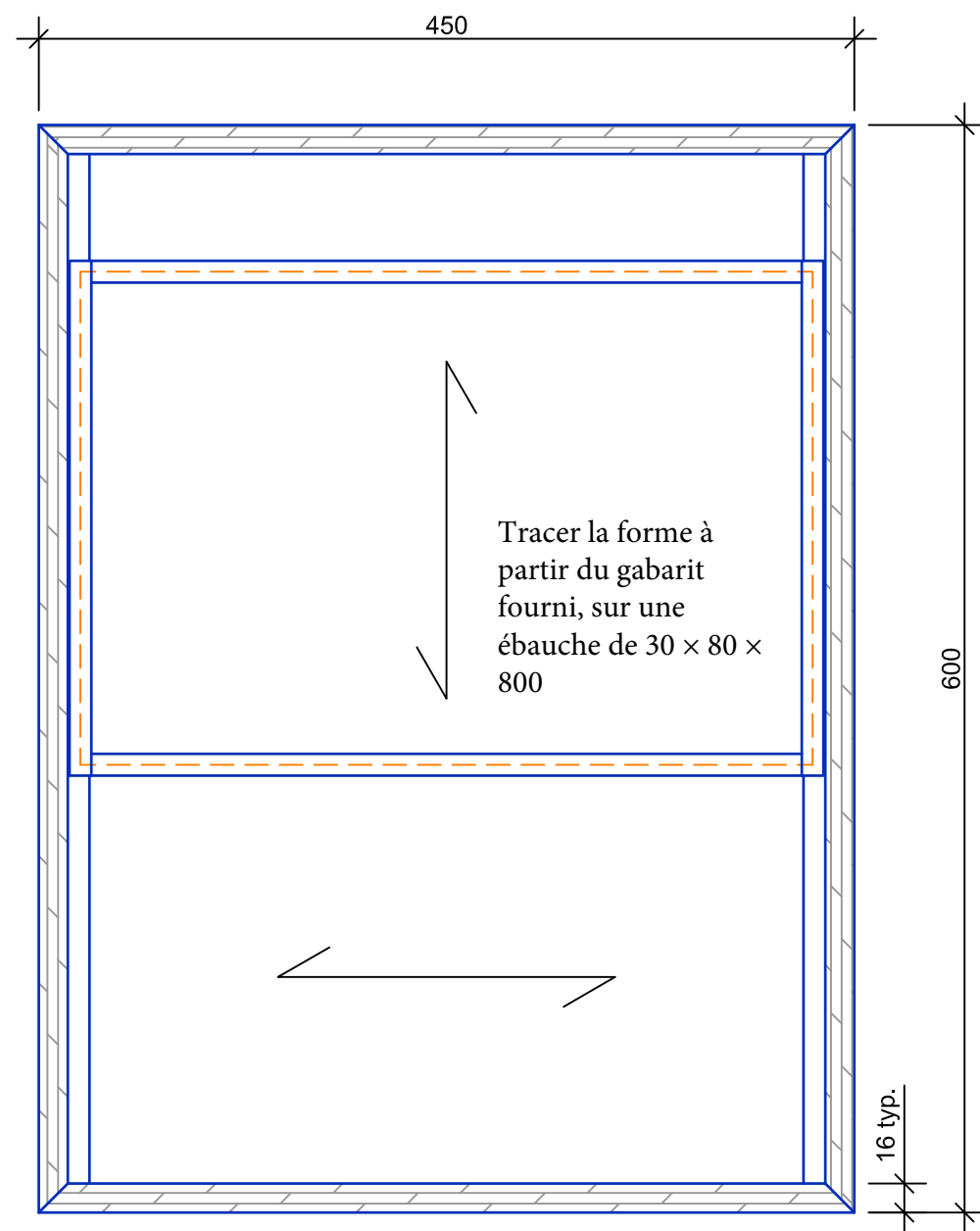
SECTION C-C
