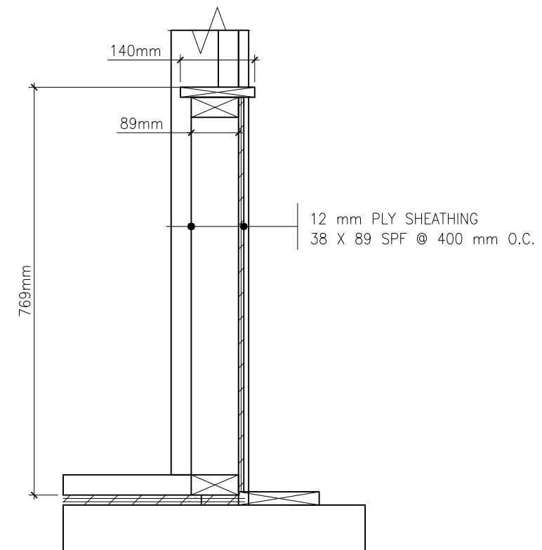
SECTION E 2 PONY WALL SCALE 1:10
