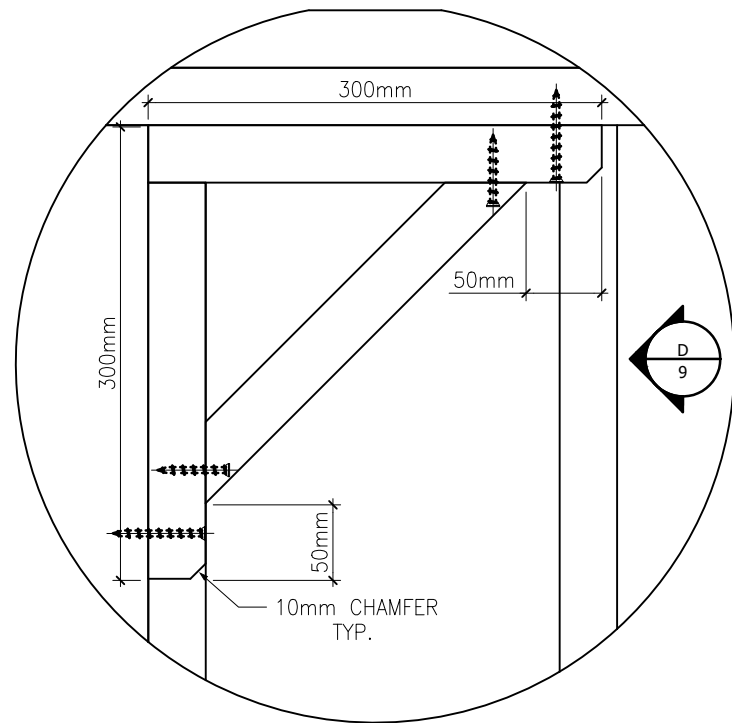
DETAIL 5 7 KNEE BRACE DETAIL SCALE 1:5
