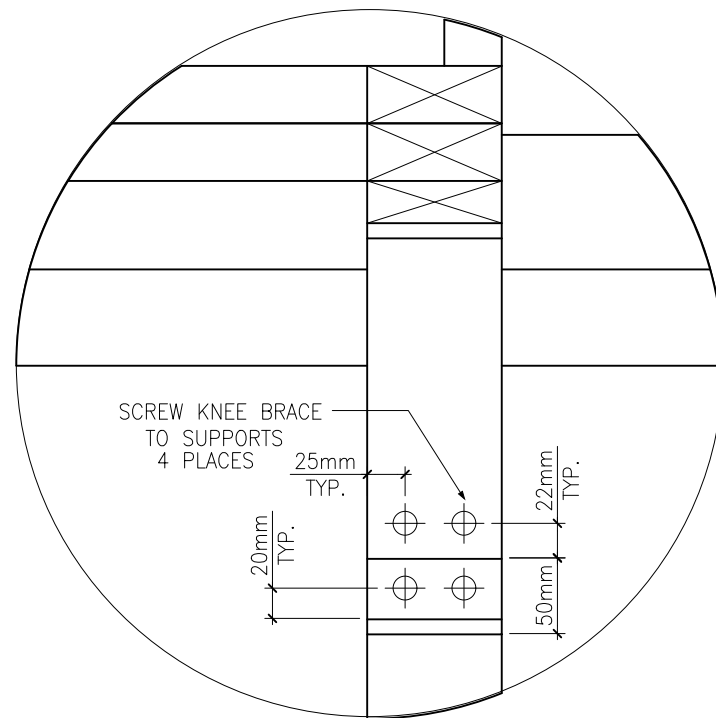
DETAIL D 9 KNEE BRACE DETAIL SCALE 1:5
