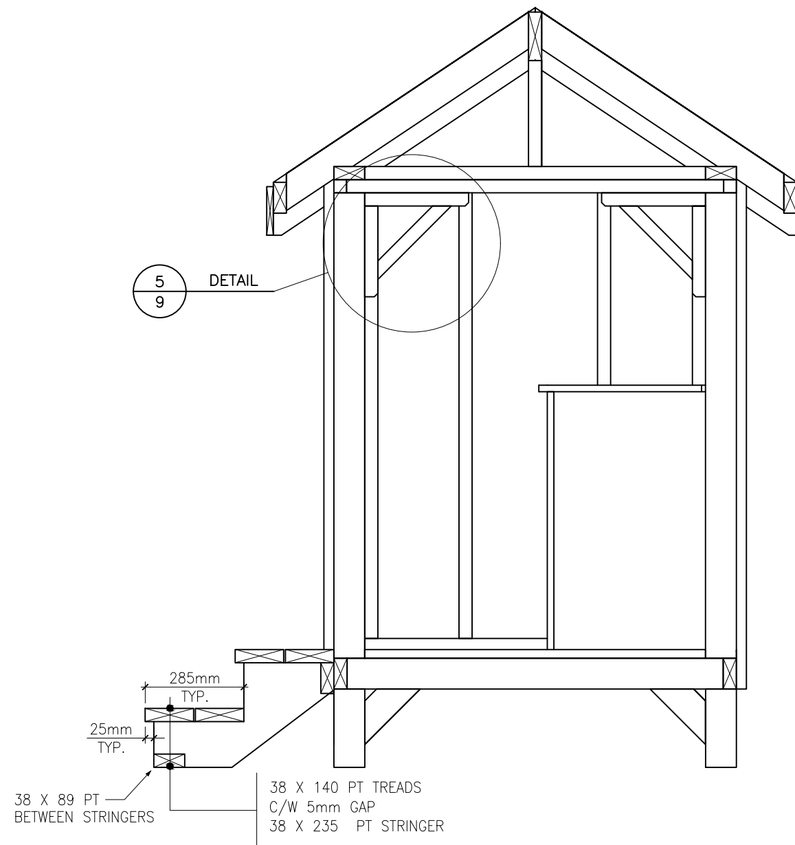
SECTION C-C SCALE 1:15
