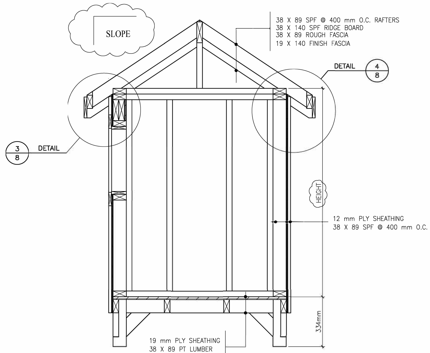
SECTION B-B SCALE 1:15
