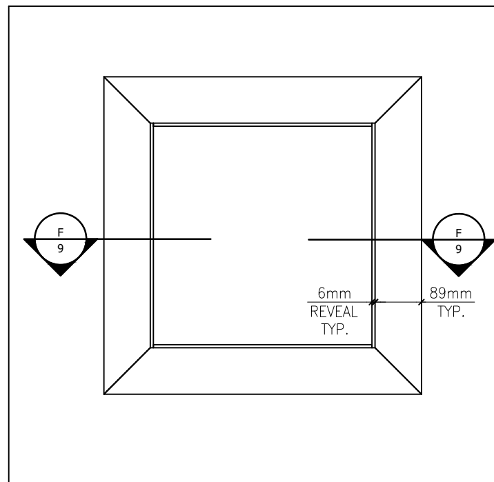
WINDOW DETAIL SCALE 1:10
