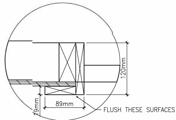
DETAIL INTERIOR WALL TRIM DETAIL TYPICAL 2 2
