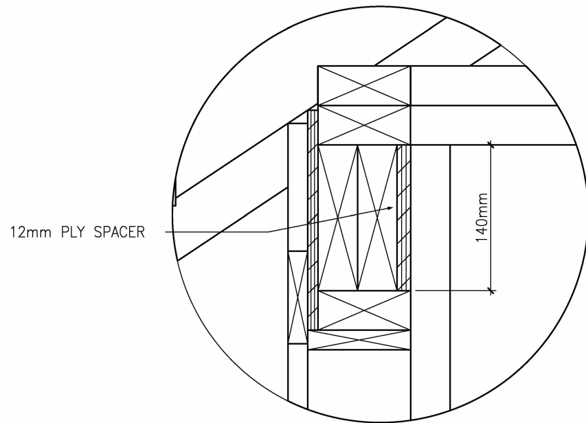
DETAIL LINTEL DETAIL 3 6
