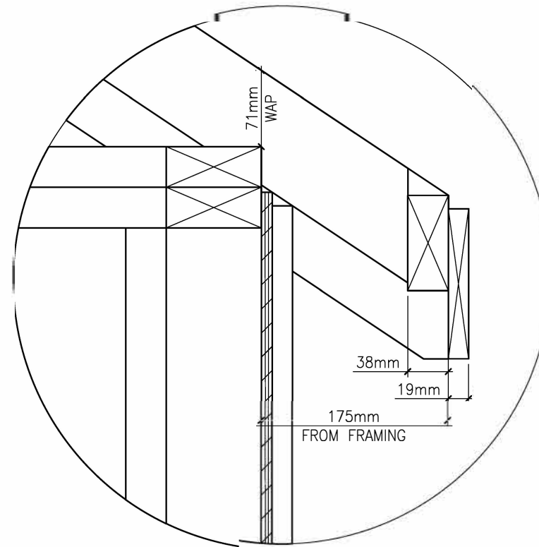
DETAIL CORNICE DETAIL 4 6
