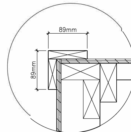
DETAIL REAR WALL TRIM DETAIL TYPICAL 1 2
