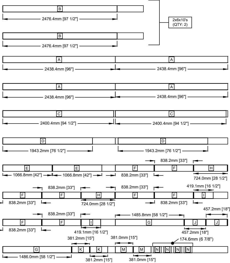
① 2x6" LUMBER DIMENSIONS SCALE = 1:40
