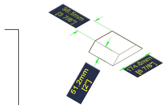
② 'N' PIECE DIMENSIONS SCALE = 1:40
