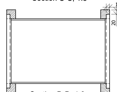
Section D-D, 1:8
