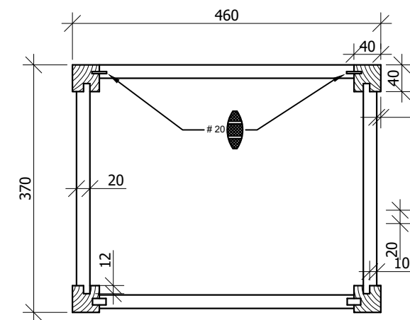
Section C-C, 1:8
