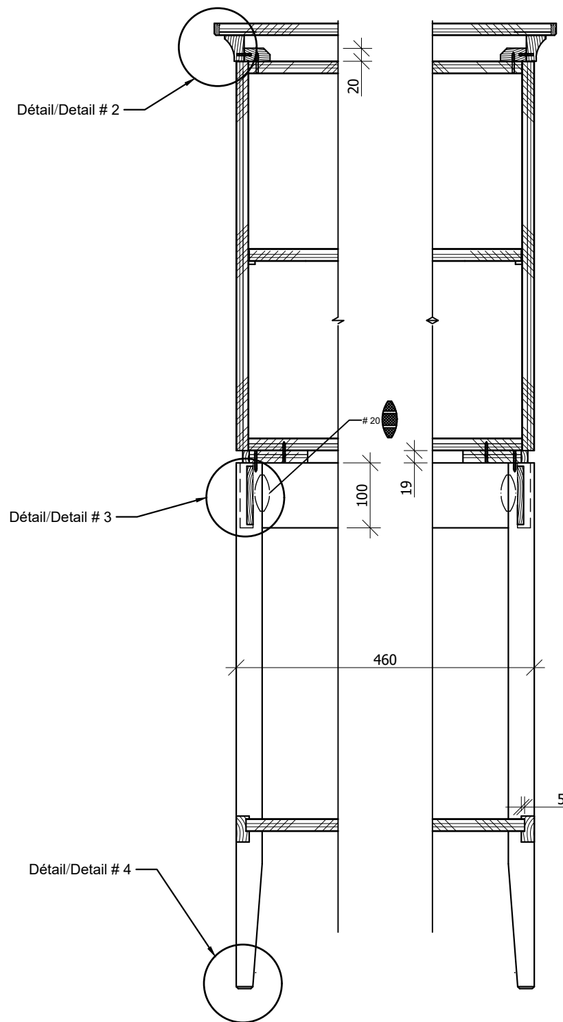
Section B-B, 1:8
