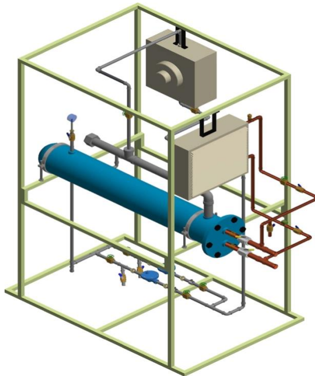
STEAM AND HOT WATER CONVERTER
