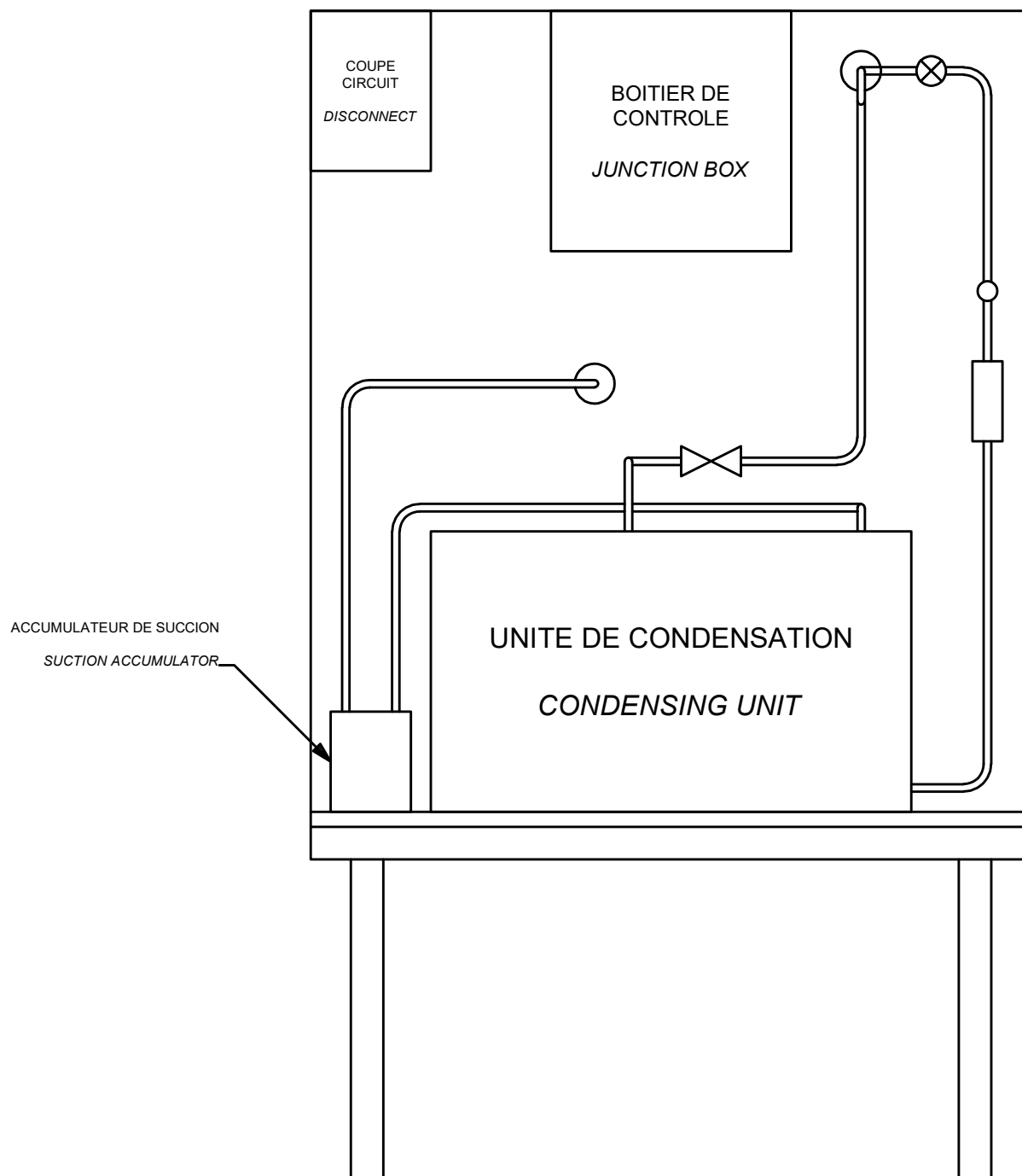
ELEVATION FRONT VIEW
