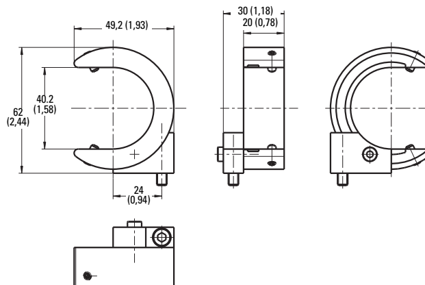
Figure 12 : Supports de montage centraux
