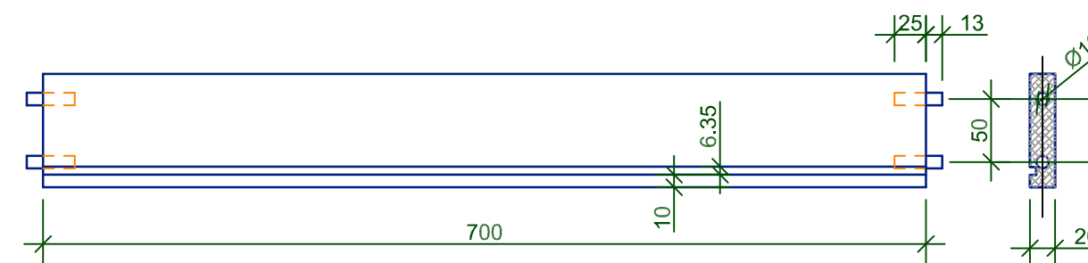
BACK RAIL
