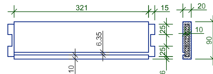
SIDE RAILS
