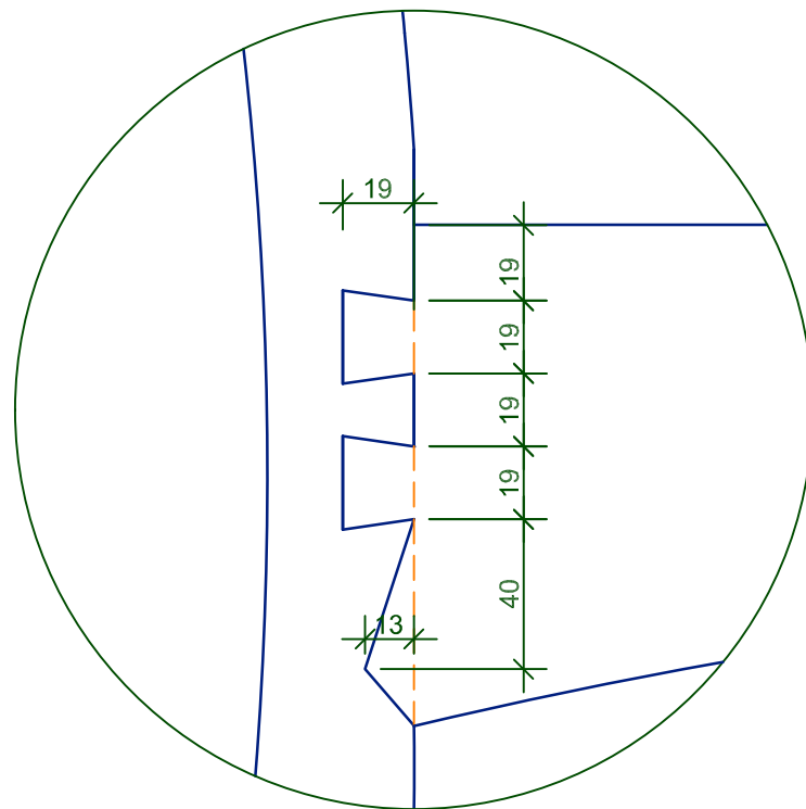
IRREGULAR DOVETAIL HALF LAP LAYOUT 1:2
