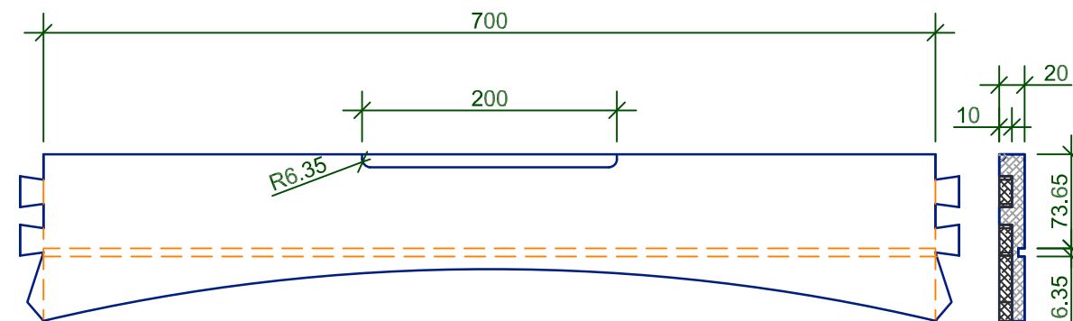
IRREGULAR DOVETAIL FRONT RAIL
