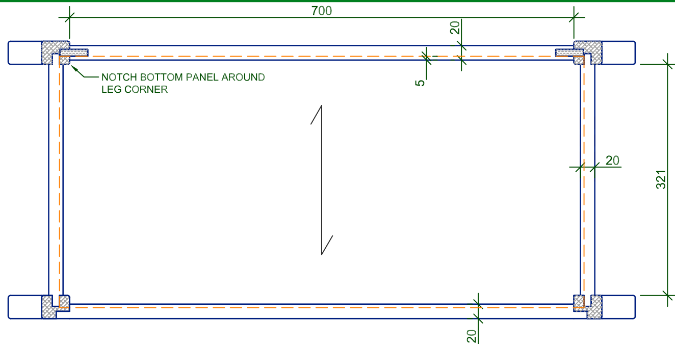
SECTION C-C
