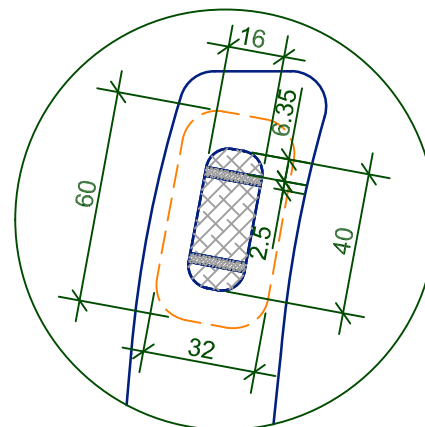
TOP RAIL OF END FRAME JOINERY DETAILS 1:2
