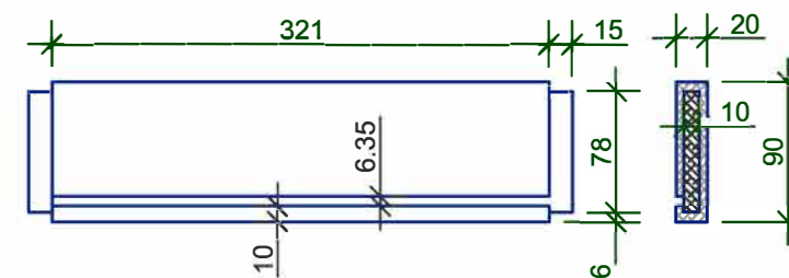
SIDE RAILS
