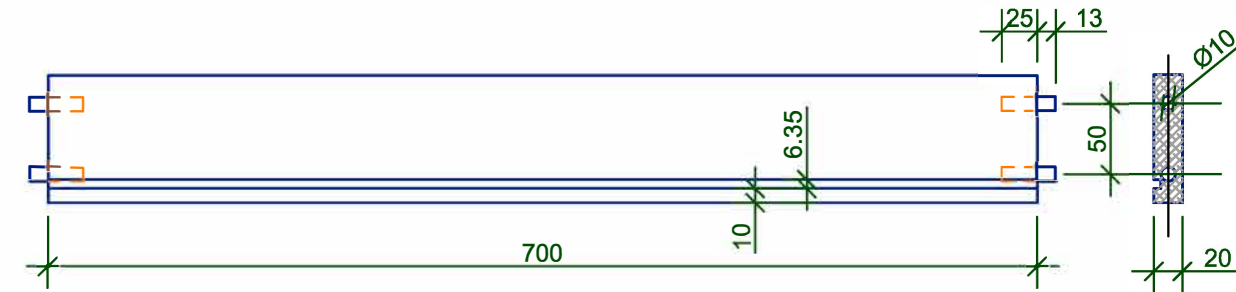
BACK RAIL
