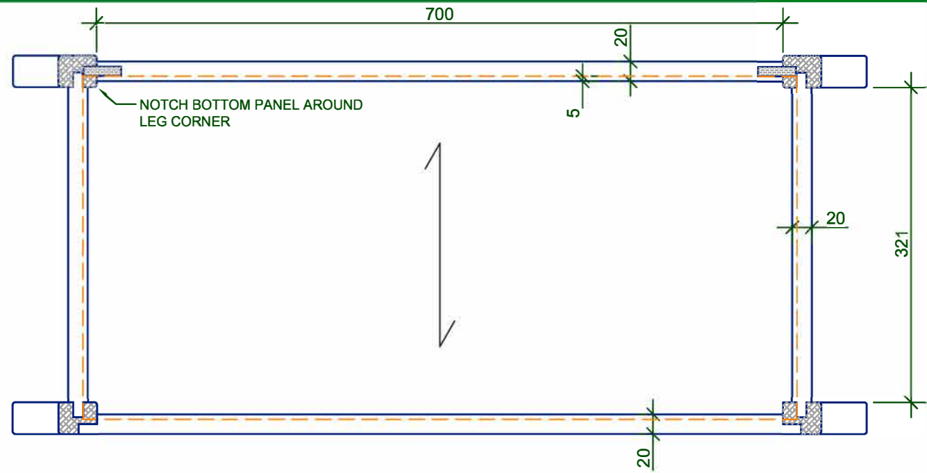
SECTION C-C
