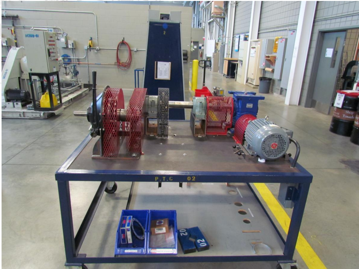
MECHANICAL ASSEMBLY STATION PROPOSED PROJECT
